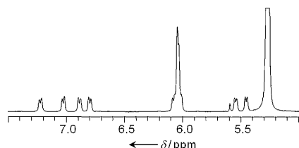
Figure 5. Aromatic region of the ^1\text{H} NMR spectrum of 2^{2+} at -50^\circ\text{C} in 3:1 \text{CD}_3\text{OD}:\text{CD}_3\text{CN} . The intense signal near \delta=5.37 ppm is the methanol OH impurity, which moves upfield as the temperature is lowered, and the small one near \delta=5.6 ppm appears to correspond to the \delta\approx 5.2 ppm peak at 20^\circ\text{C} (see Supporting information for details).
